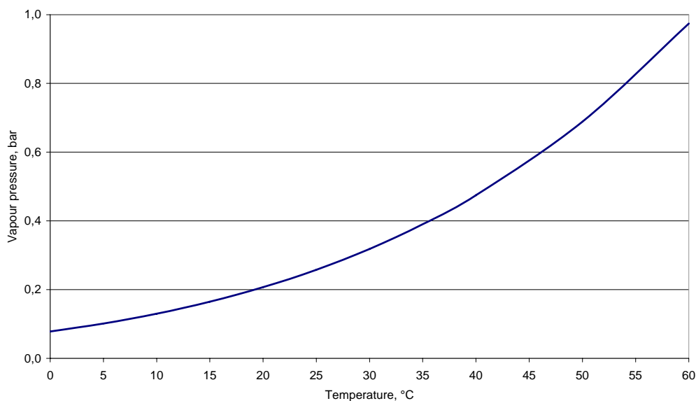
Vapour pressure of chloroform
